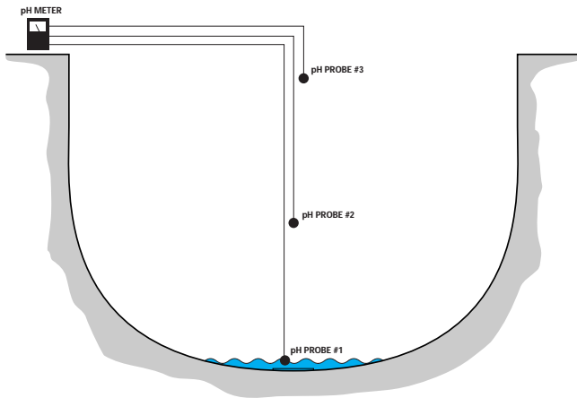
Figure 2 – Cutaway View of Swimming Pool with pH Probes in Place and Water Level at 6 Inches
