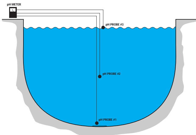
Figure 4 – Cutaway View of Swimming Pool with pH Probes in Place and Water Level at 6 Feet
