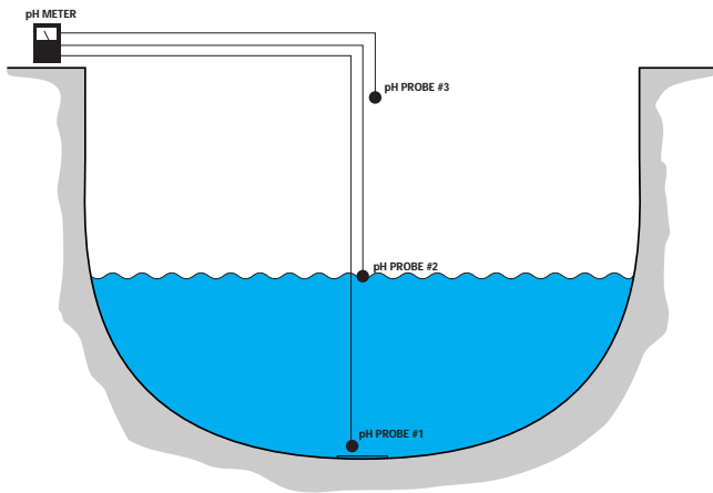
Figure 3 – Cutaway View of Swimming Pool with pH Probes in Place and Water Level at 3 Feet
