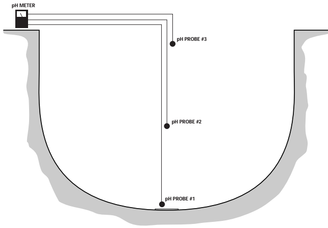
Figure 1 – Cutaway View of Swimming Pool with pH Probes in Place
